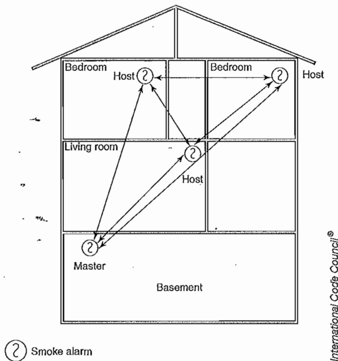
Smoke alarm location and interconnection
