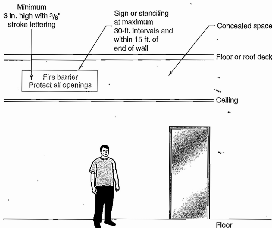
Identification sign for fire barrier
