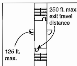
Egress requirements from individual R-2 dwelling units
