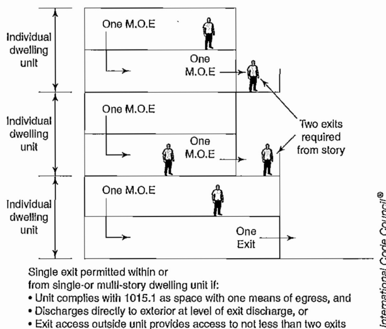
Egress from multistory dwelling units
