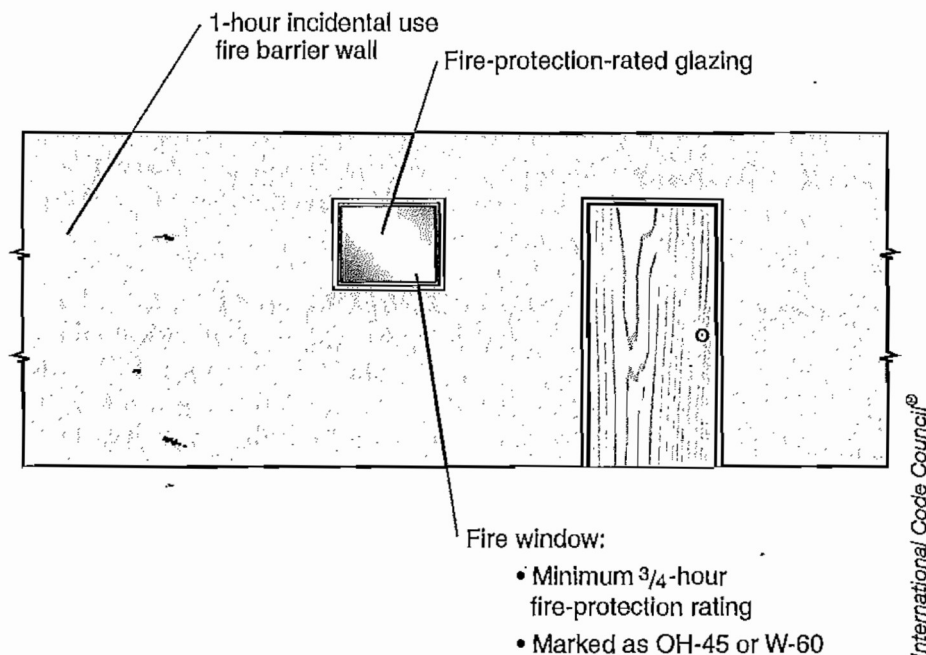
Fire window in incidental-use fire barrier wall
