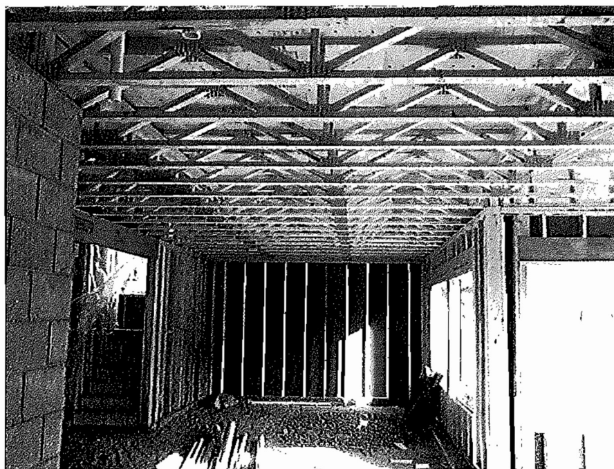
Open web floor trusses require a fire protection membrane applied to the underside.
