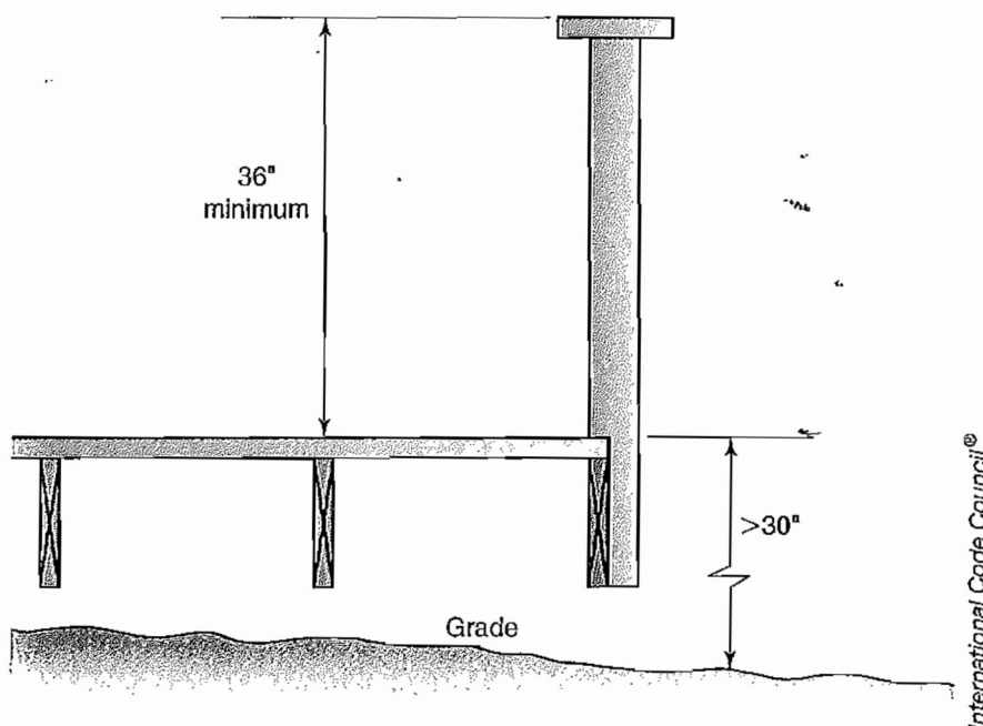
Minimum residential guard height
