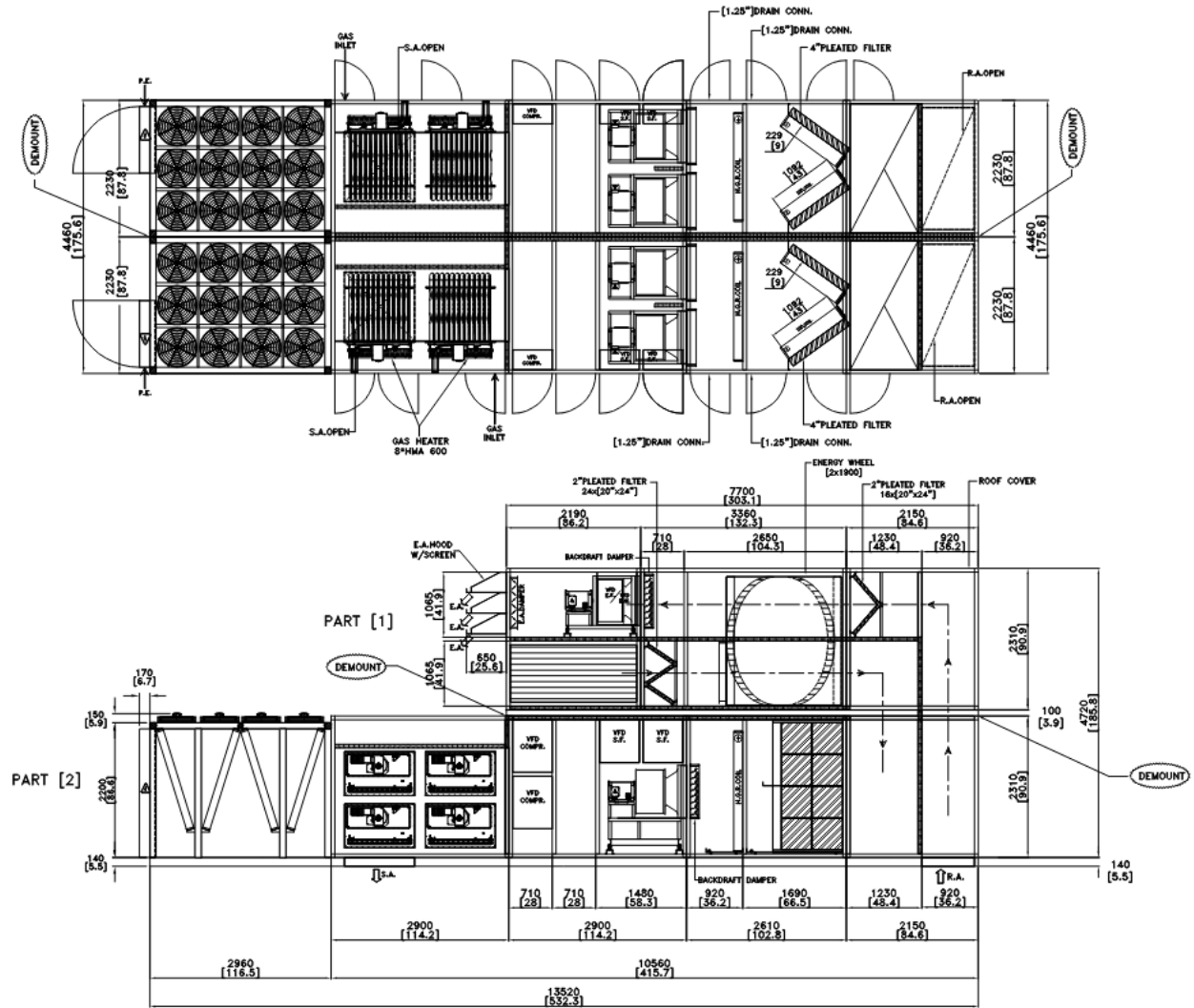
Figure 4 - Custom RTU arrangement provided by vendor
