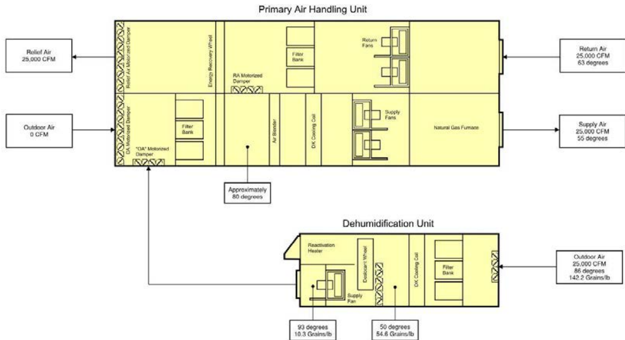
Figure 5 – Dehumidification coupled with primary air-handling Unit (ice event)
