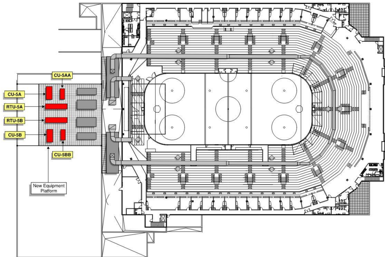
Figure 7 - Proposed RTU-5 Upgrades
