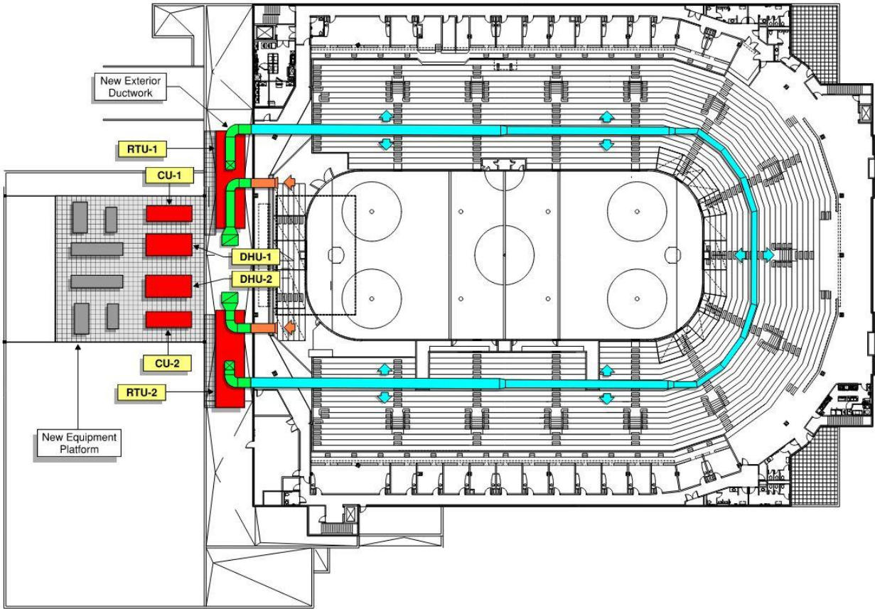
Figure 3- Proposed RTU-1 and RTU-2 Replacement Strategy
