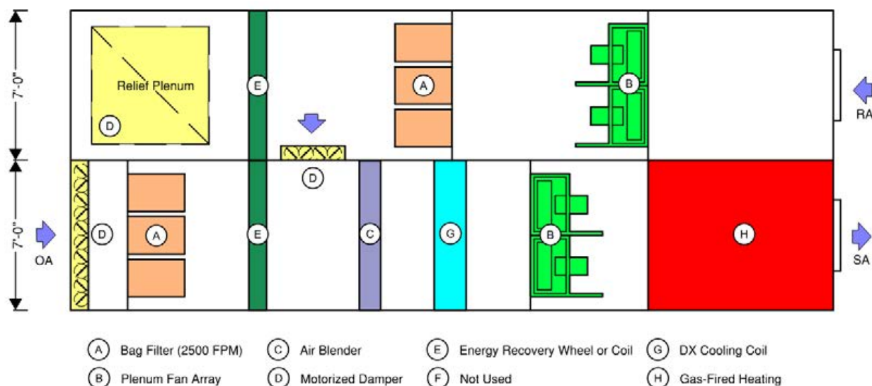
Figure 2- Conceptual Rooftop Air-handling Unit Configuration
