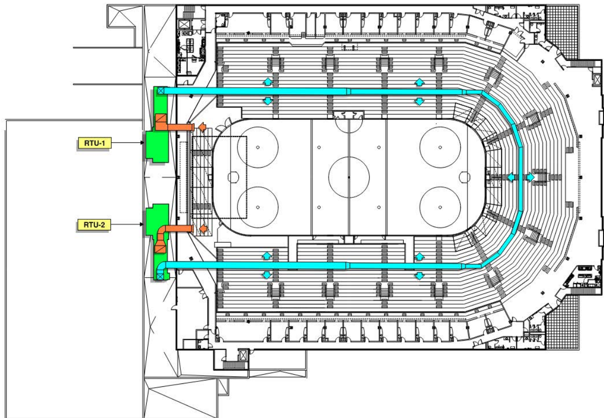
Figure 1 - Existing RTU-1 and RTU-2 Configuration
