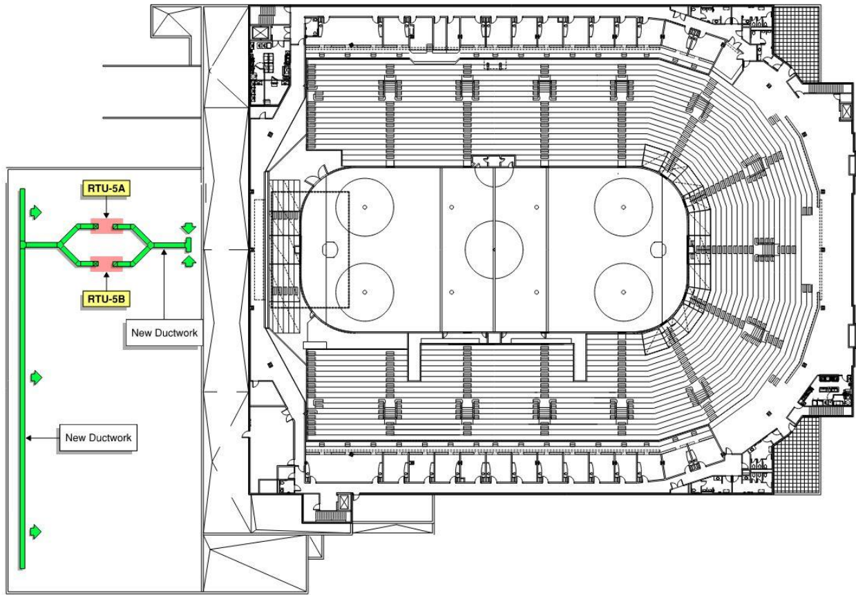
Figure 8 - New ductwork arrangement in Ice Center
