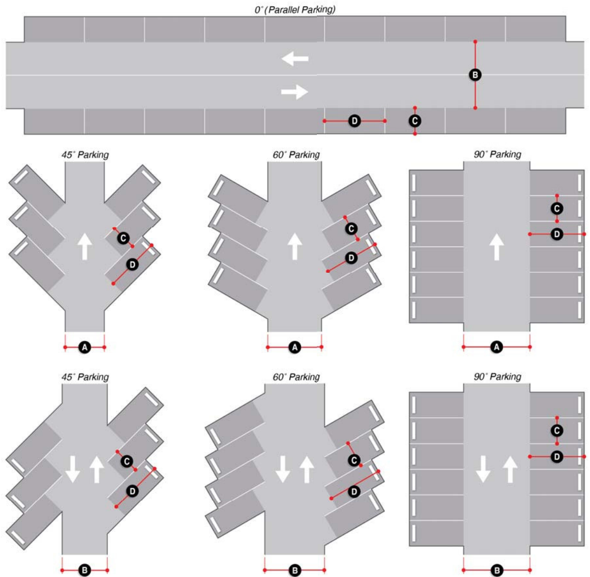
Diagram 1206 Dimensional Standards for Parking Spaces and Aisles
