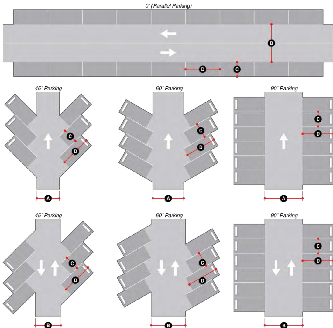
Dimensional Standards for Parking Spaces and Aisles
